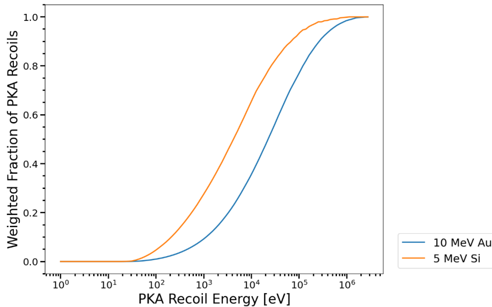
Figure 12: Weighted cumulative PKA energy spectra for 10 MeV Au and 5 MeV Si in SiC, 530 ions used for both. All other setting left as their defaults.
